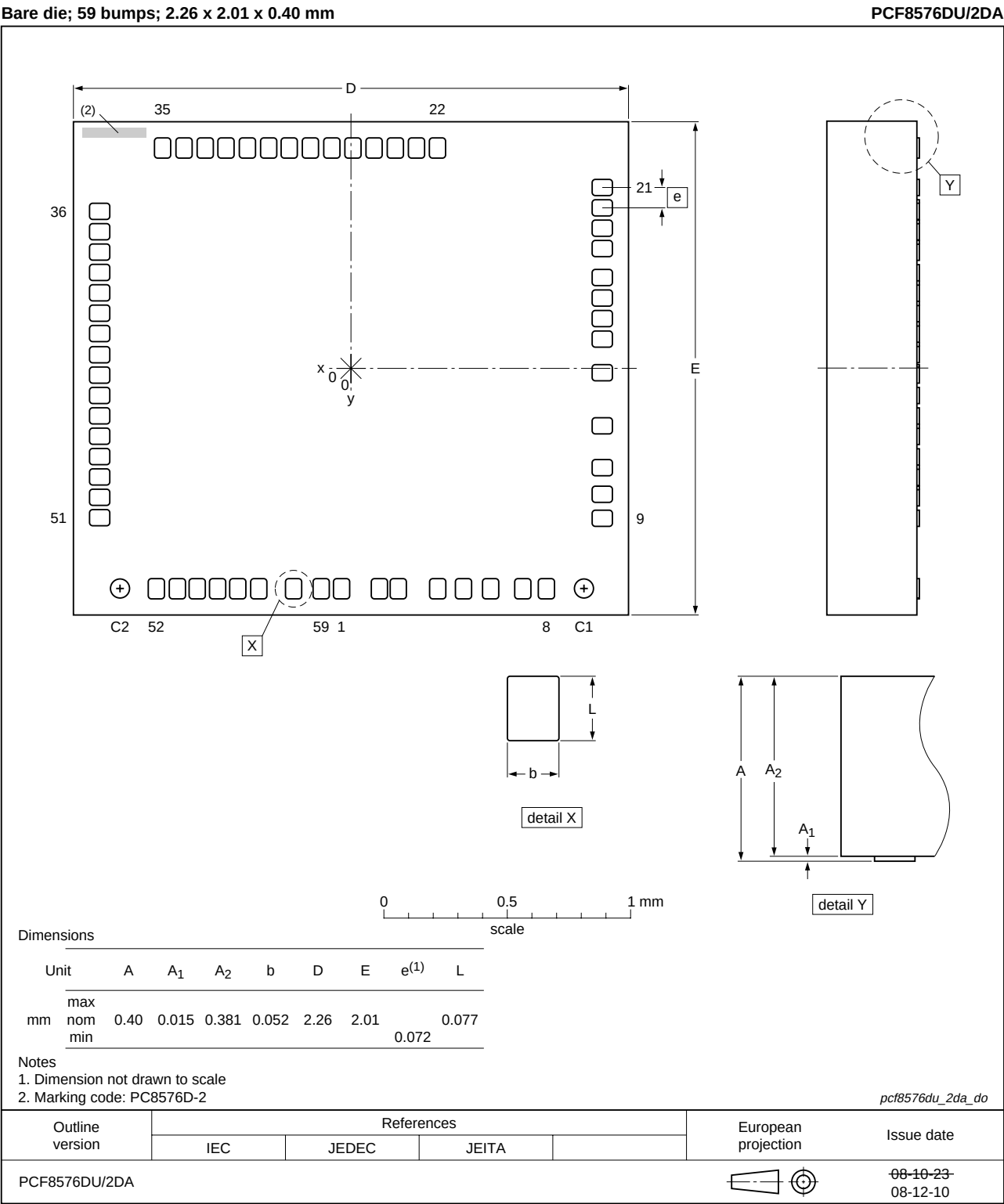
Fig 27. Bare die outline PCF8576DU/2DA/2 PCF8576D_7 © NXP B.V. 2008. All rights reserved. Product data sheet Rev. 7 — 18 December 2008 39 of 52
